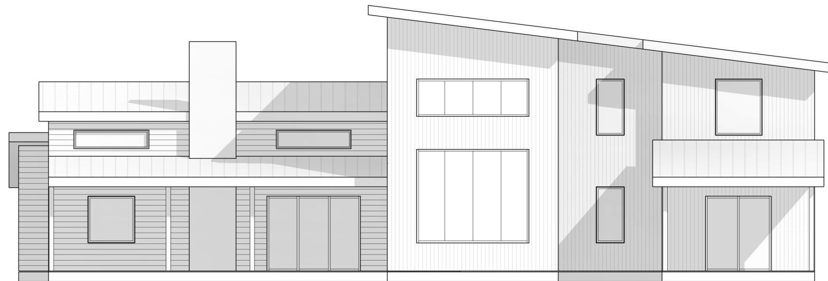
1 Elev_Array_Back 1" = 10'-0"
